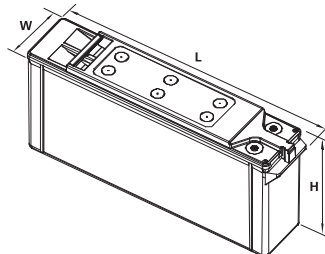
12V101F
